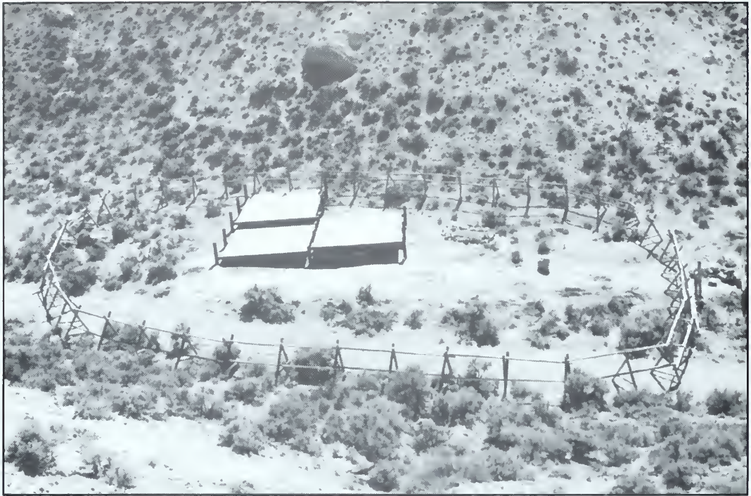
Photo 11. Completed big game guzzler in northern Nevada, consisting of water collecting aprons, buried tanks, drinker surrounded by rocks, and buck-and-rail fence.
